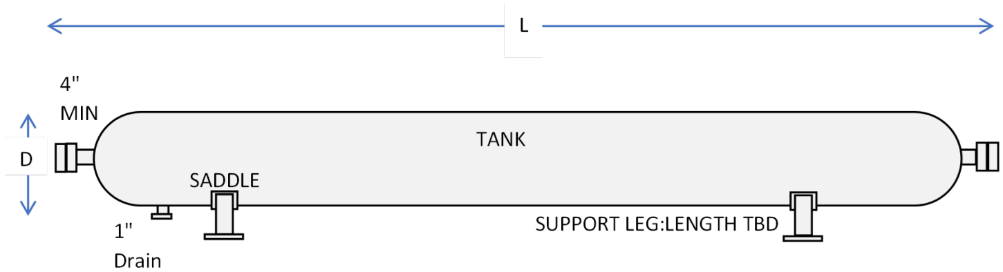
1- Individual Tank configuration
