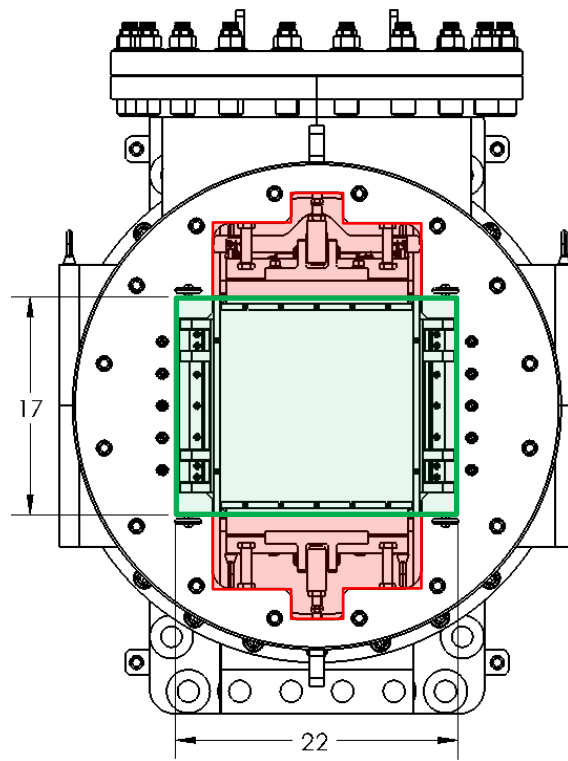
Figure 1: Downstream face of transonic test section showing – red) zone to be blocked off by transition section, green) minimum required area of transition section inlet plane
