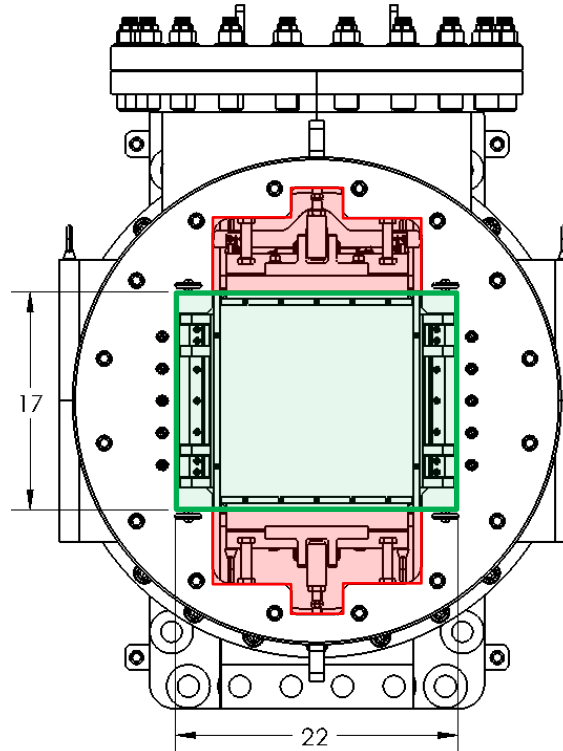
Figure 2: Downstream face of transonic test section showing – red) zone to be blocked off by transition section, green) minimum required area of transition section inlet plane
