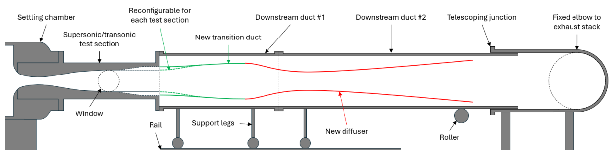
Figure 1: Schematic diagram of a notional diffuser for APWT.
