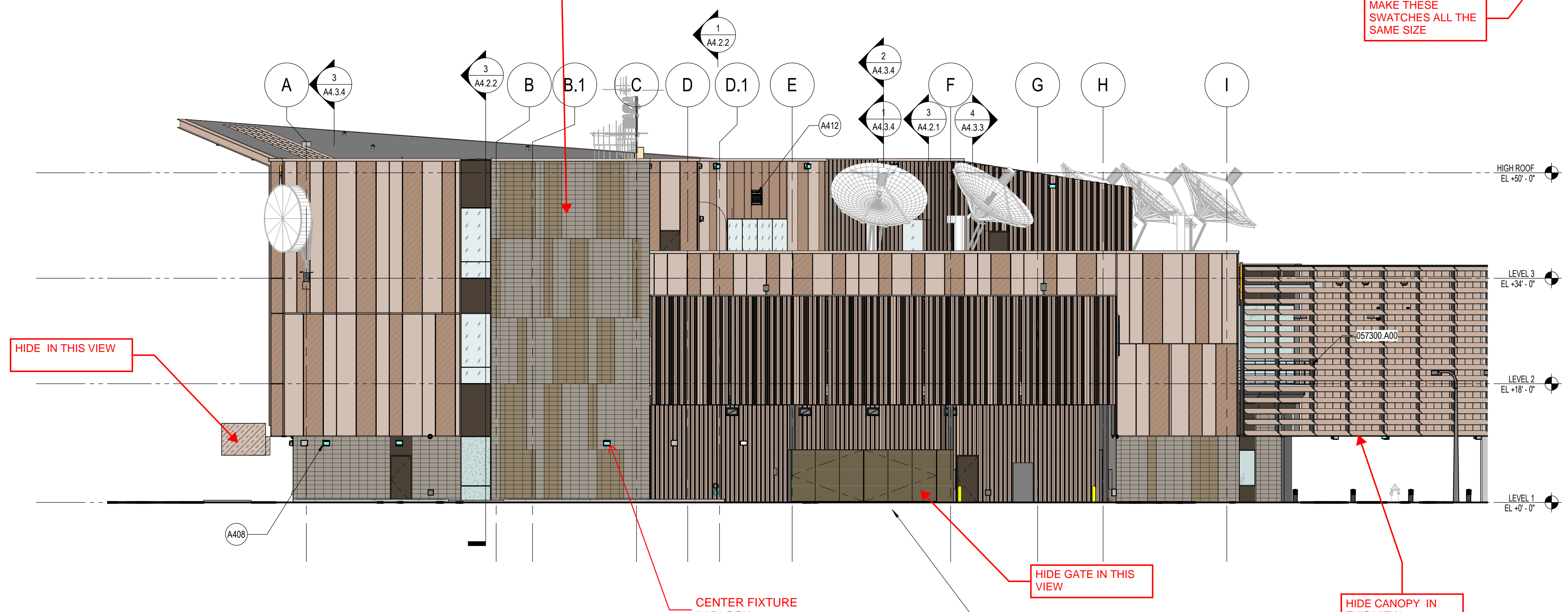
2 BUILDING ELEVATION - WEST (CANOPY & SITE WALLS NOT SHOWN) SCALE: 3/32" = 1'-0"
