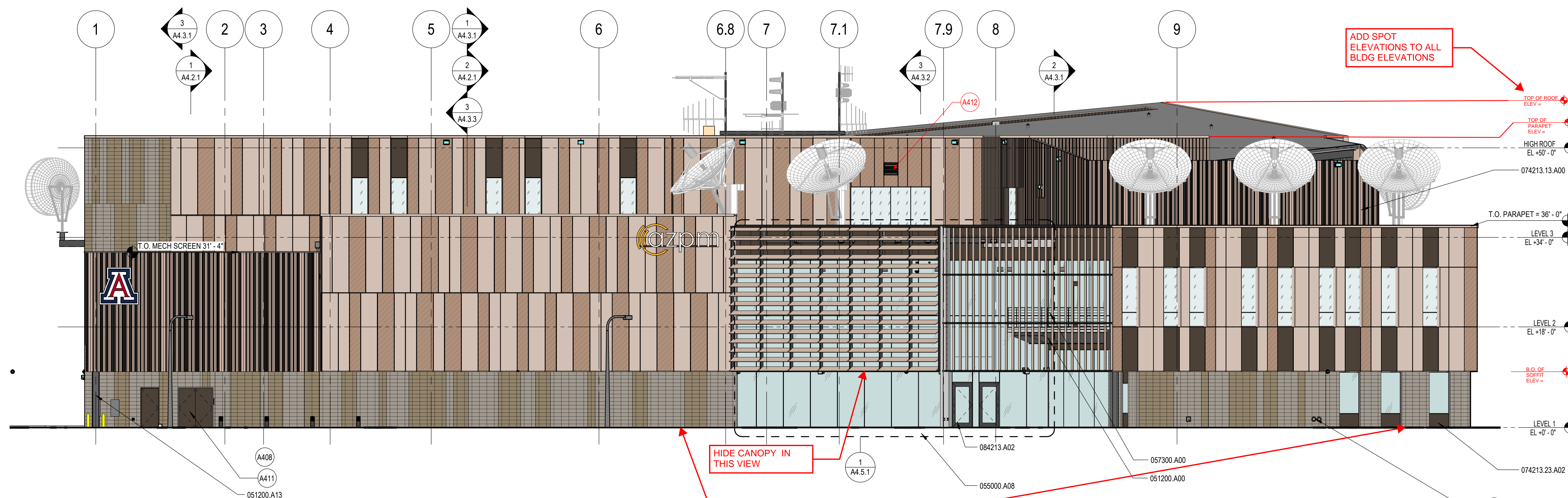
3 BUILDING ELEVATION - SOUTH (CANOPY & SITE WALLS NOT SHOWN) SCALE: 3/32" = 1'-0"
