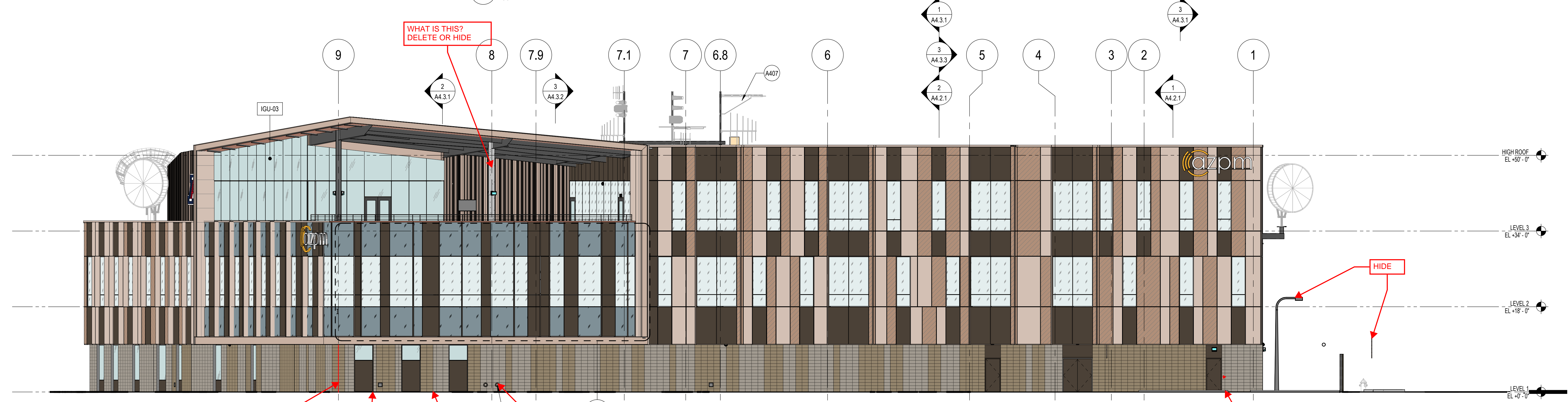
2 BUILDING ELEVATION - WEST (CANOPY & SITE WALLS NOT SHOWN) SCALE: 3/32" = 1'-0"
